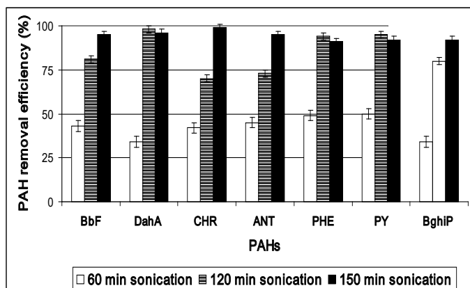
Figure 1: Effect of increasing sonication time on PAHs removal efficiencies at 60^\circ\text{C} (sonication power=640 W, sonication frequency=35 kHz).
