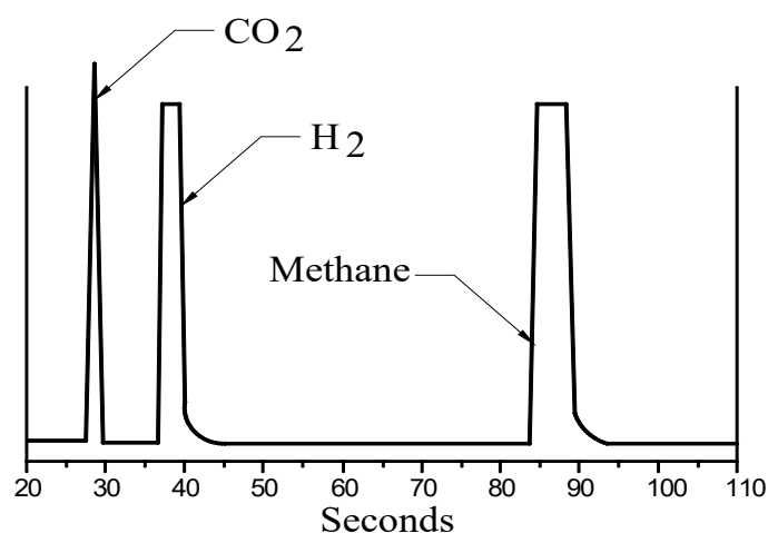
Figure 2: \text{CH}_4(\text{g}) , \text{H}_2(\text{g}) and \text{CO}_2(\text{g}) spectra measured in the headspace of the sonicator by GC (sonication power=640 W, sonication frequency=35 kHz).
