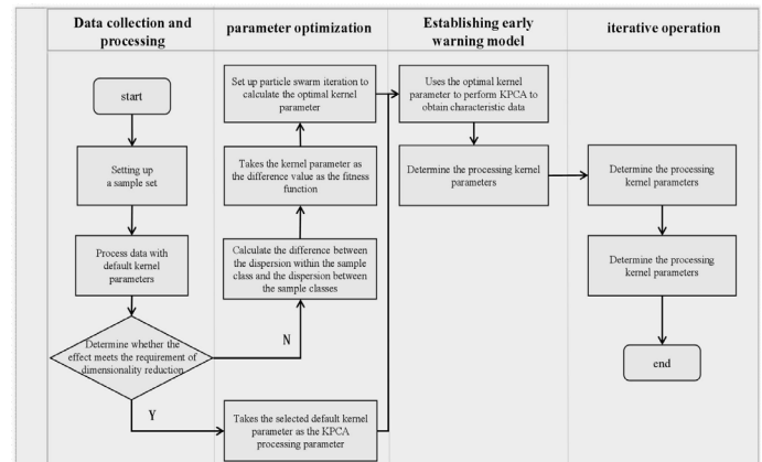
Figure 1: Algorithm Flow chart.
