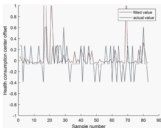
Figure 5: Traditional PCA-Regression consumption curve.
